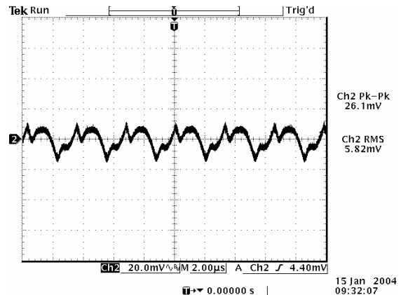
Ripple and noise at full load, V_{in}=5.0\text{ V} , V_o=1.8\text{ V}
