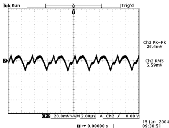
Ripple and noise at full load, V_{in}=5.0\text{ V} , V_o=1.5\text{ V}
