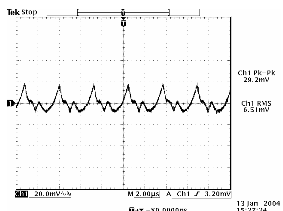
Ripple and noise at full load, V_{in}=5.0\text{ V} , V_o=3.3\text{ V}
